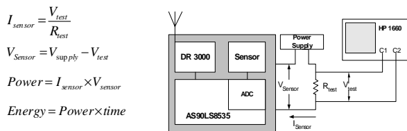
Figure 17: Power and Energy Relationships and Measurement Setup
